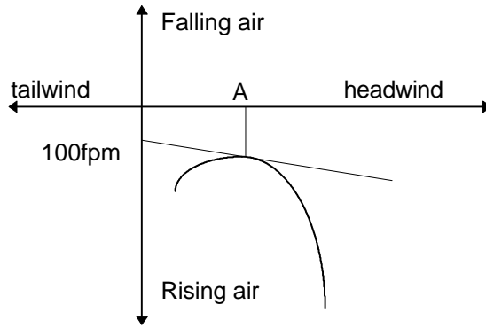
Figure 12 Polar curve with thermal
