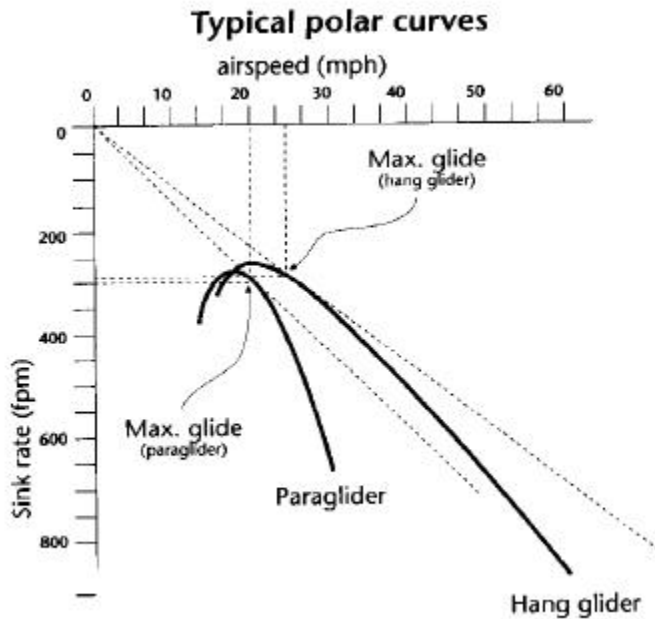
Figure 10 Polar curves
