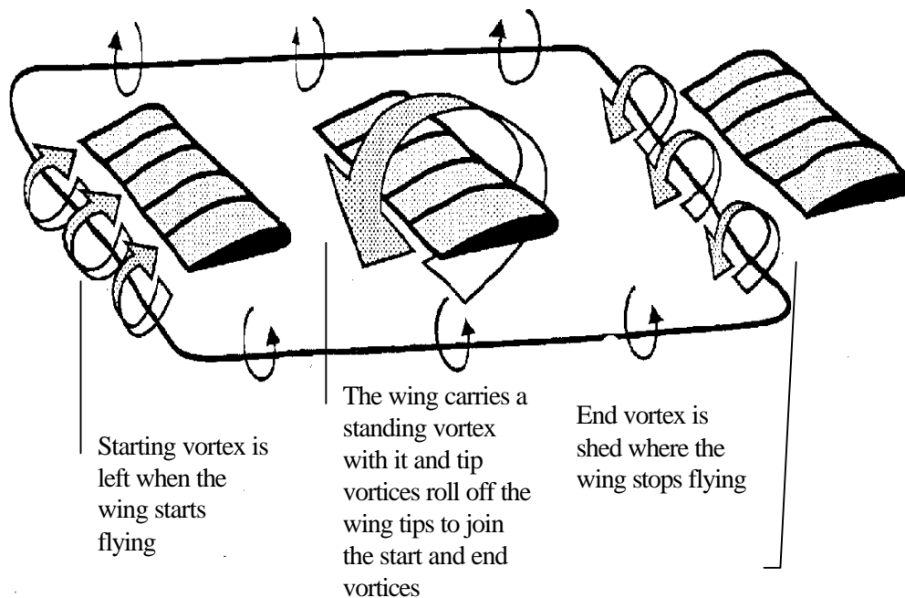
Figure 3 Vortices
