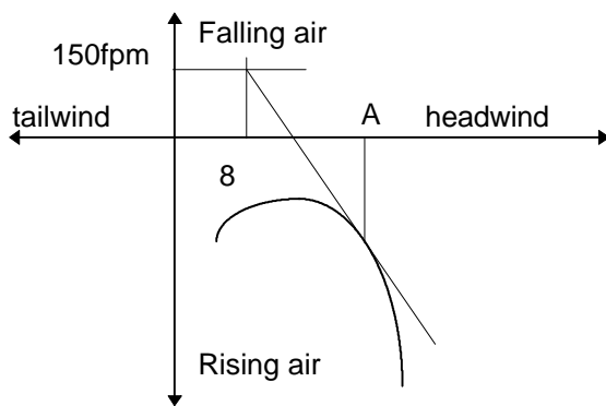
Figure 13 Polar curve with both
