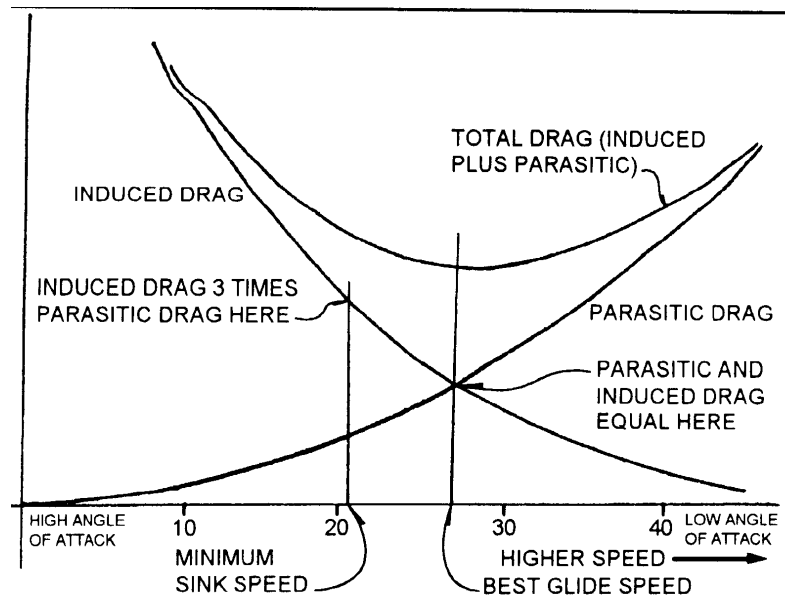
Figure 9 Total drag
