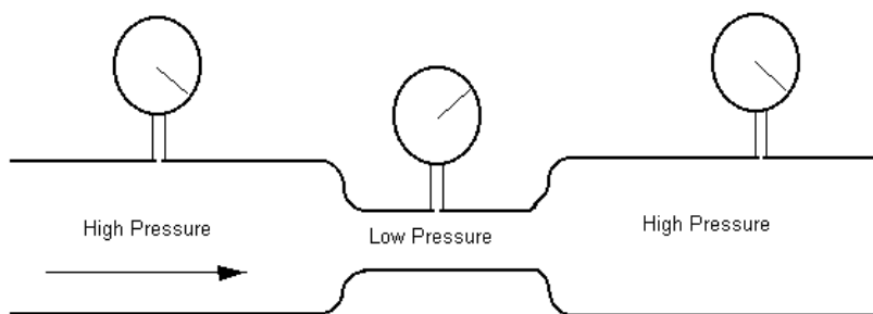
Venturi Tube demonstrates Bernoulli principle
