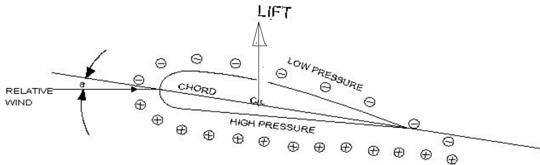
Figure 2 Lift on the airfoil
