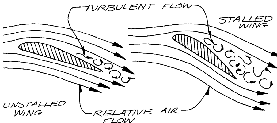
Figure 4 Stall effects
