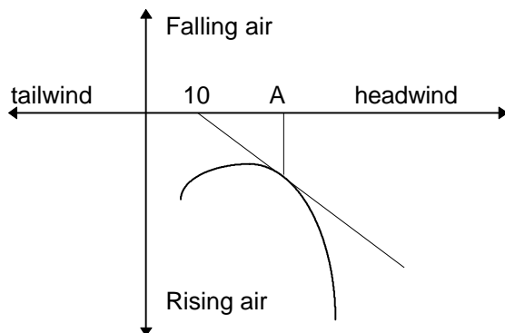
Figure 11 Polar curve with headwind
