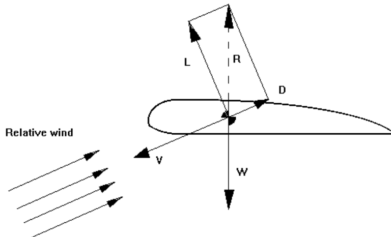
Figure 8 Forces on a glider
